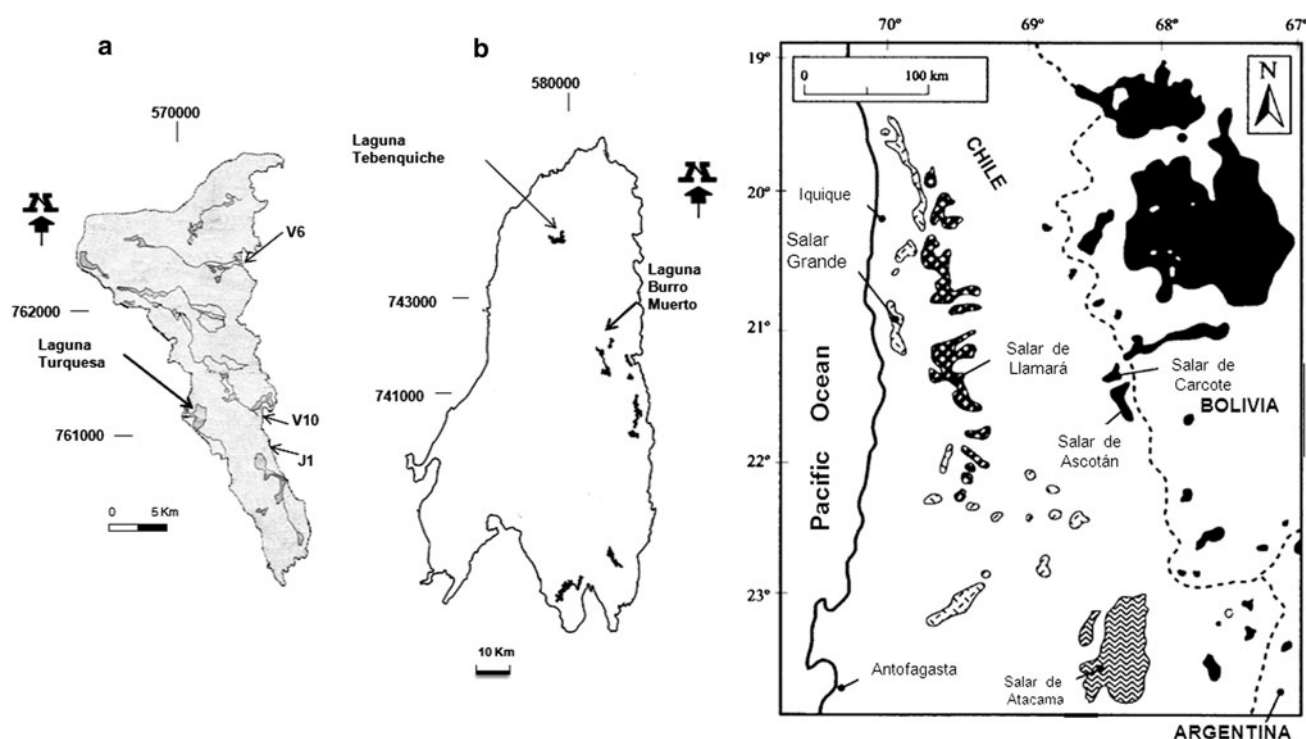
Fig. 1 Map of Salar de Ascotán ( left ), showing the location of Laguna Turquesa, J1, V6 and V10, and Salar de Atacama ( middle ) showing the location of Laguna Burro Muerto and Tebenquiche. Inset the salt flats sampled are shown in a map of Northern Chile ( right )
